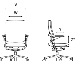
XENIUM OPERATIVE UPH ESP-ST R36 Weight | Waga 17.20 kg
