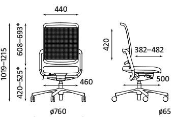
XENIUM OPERATIVE MESH ESP-ST Weight | Waga 13.90 kg
