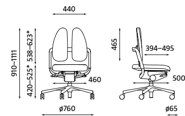
XENIUM OPERATIVE DUO-BACK DNP-ST Weight | Waga 18.20 kg
