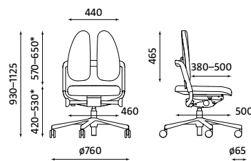
XENIUM OPERATIVE DUO-BACK IND-ST Weight | Waga 16.50 kg
