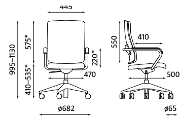
XENIUM X-CROSS UPH Weight | Waga 14.00 kg
