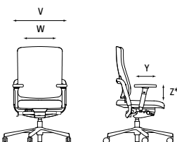
XENIUM OPERATIVE UPH ESP-ST R37 Weight | Waga 17.20 kg
