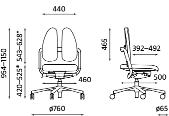
XENIUM OPERATIVE DUO-BACK ESP-ST Weight | Waga 16.20 kg
