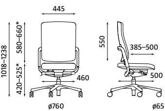
XENIUM OPERATIVE UPH ESP-ST Weight | Waga 16.20 kg
