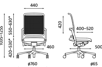
XENIUM OPERATIVE MESH IND-ST Weight | Waga 16.00 kg
