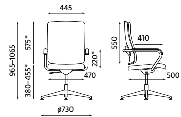
XENIUM X-CROSS UPH ST54 Weight | Waga 14.00 kg
