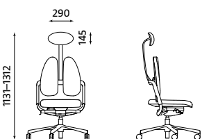
XENIUM OPERATIVE DUO-BACK ESP-ST HRUA Weight | Waga 16.90 kg
