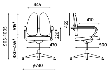
XENIUM X-CROSS DUO-BACK ST54 Weight | Waga 14.20 kg
