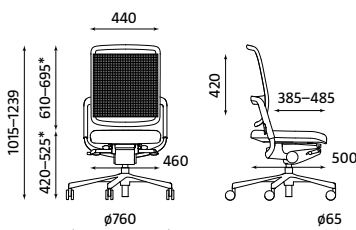
XENIUM OPERATIVE MESH DNP-ST Weight | Waga 15.90 kg
