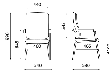
XENIUM FRAME 4L UPH Weight | Waga 10.00 kg
