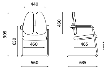
XENIUM FRAME CF DUO-BACK Weight | Waga 9.00 kg
