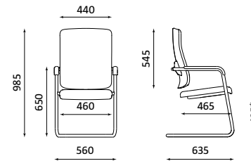
XENIUM FRAME CF UPH Weight | Waga 10.00 kg
