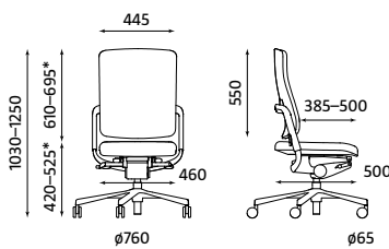
XENIUM OPERATIVE UPH DNP-ST Weight | Waga 17.70 kg
