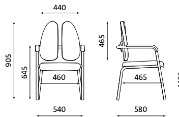
XENIUM FRAME 4L DUO-BACK Weight | Waga 9.00 kg
