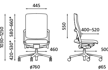
XENIUM OPERATIVE UPH IND-ST Weight | Waga 16.00 kg
