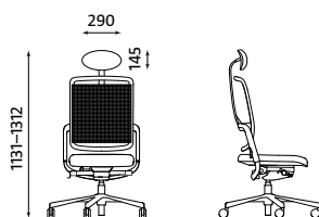
XENIUM OPERATIVE MESH ESP-ST HRUA Weight | Waga 14.60 kg
