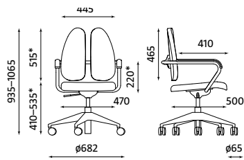
XENIUM X-CROSS DUO-BACK Weight | Waga 14.20 kg
